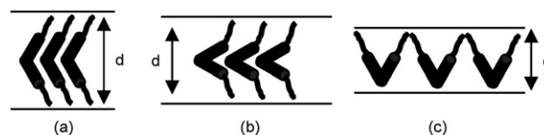
Fig. 4 Different schematic drawings of the molecules proposed for the SmA mesophase induced by bent-core molecules: for a SmAP mesophase (a) and for a calamitic SmA mesophase (b, c) (any polar arrangement is proposed in this case).
