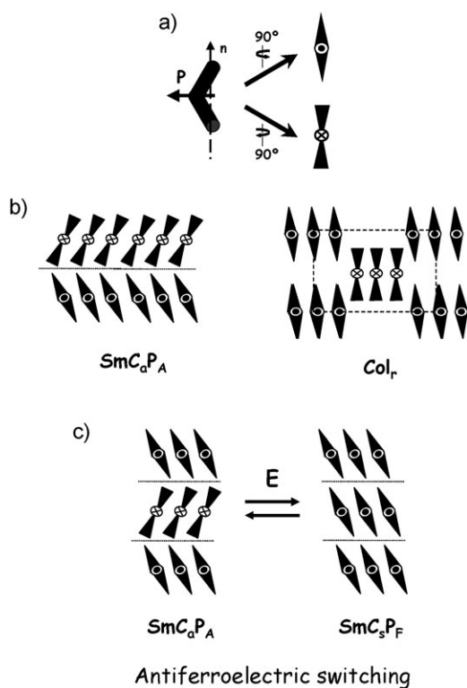
Fig. 2 Schematic representations used for bent-shaped molecules (a). Models proposed for some of the arrangements, in the SmCP and Col r packings (b). Schematic representations of the antiferroelectric switching of a SmC a P A and SmC s P F mesophase induced by applying an electric field (c).
