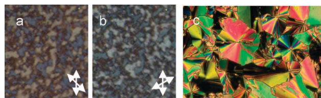
Fig. 6 Photomicrographs of the texture of (a) SmCP phase of compound CO at 180 °C when uncrossing polarizers (a) left and (b) right. (c) columnar mesophase of compound S at 152 °C.
