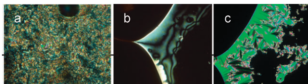
Fig. 3 Photomicrographs of the textures of the (a) SmCP phase of N(1,6) at 146 °C and of the nematic (b) and SmA (c) phases of N(2,3) at 210 and 207 °C, respectively, between glass plates.
