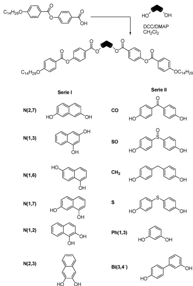
Scheme 1 The synthetic route and the schematic representation of the two series of bent-shaped compounds studied.
